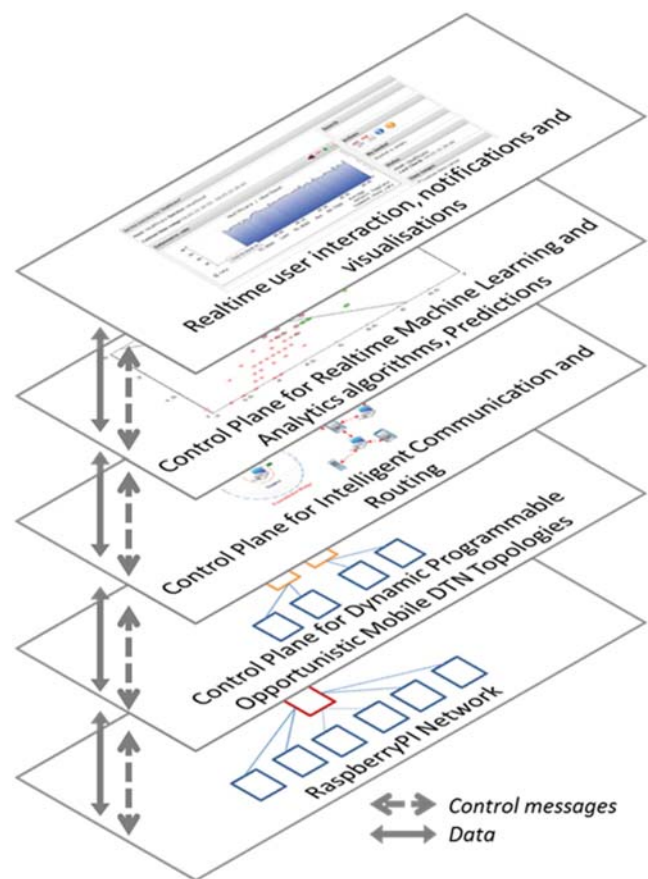
FIGURE 1. Overview of the layered architecture of MODiToNeS.
